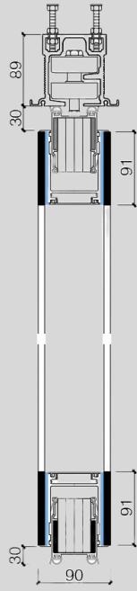
Section Detail
