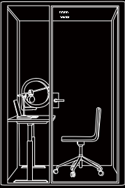
W1575*D1200*H2200mm
