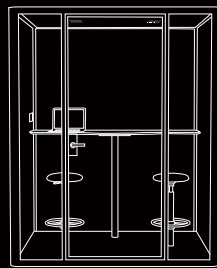
W1750*D1200*H2200mm
